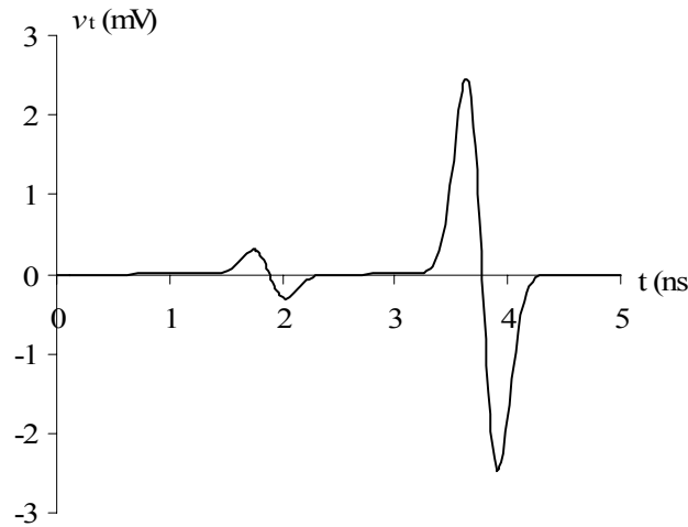
Figure 4.14 Reflected Voltage vs. Time (2 Slots Spacing at 0.5 m)
