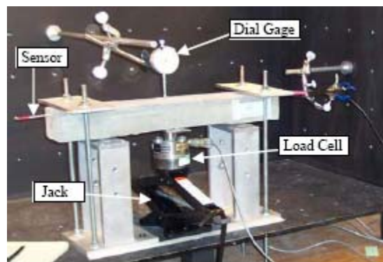
Figure 6.4 Three-point Bending Test of a Simply-Supported Beam
