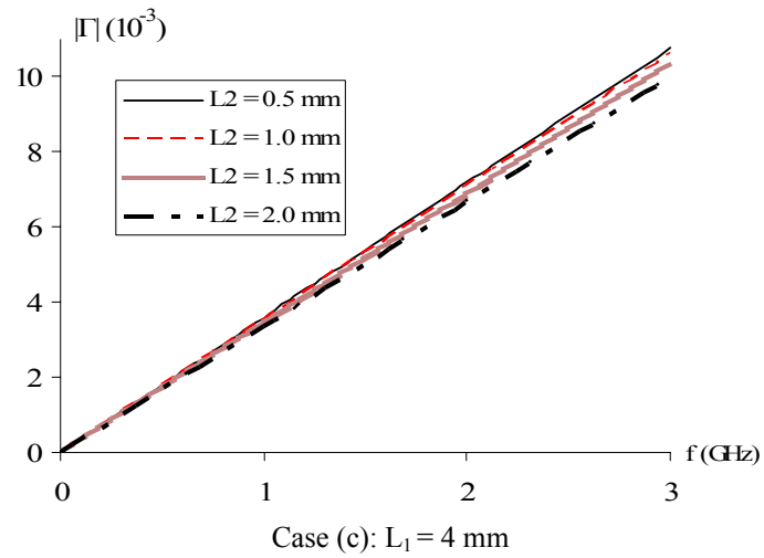
Figure 4.11 Reflection Coefficient vs. Frequency
