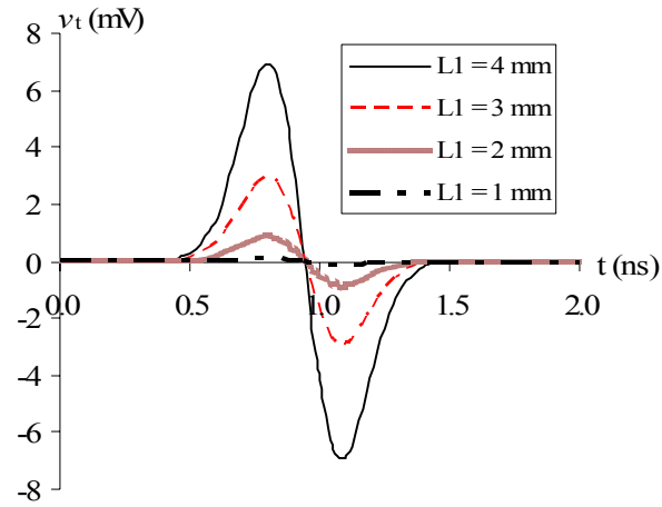
Case (a): L_1/L_2 = 10
