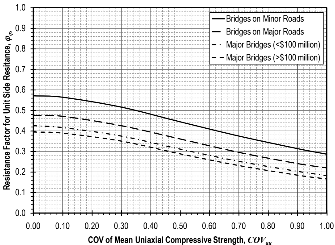
Figure 751.37.3.1 Resistance factors for unit side resistance of drilled shafts in rock from uniaxial compression tests on intact rock core.
