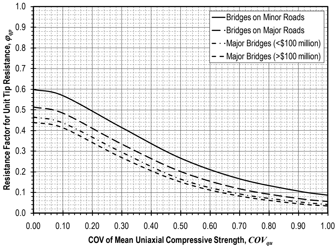
Figure 751.37.3.2 Resistance factors for unit tip resistance of drilled shafts in rock from uniaxial compression tests on intact rock core.
