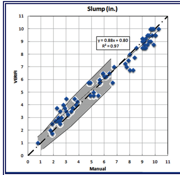
Figure 2. Manual slump measurement vs. Verifi measurement (acceptable precision in ASTM C143 are shown in gray)
