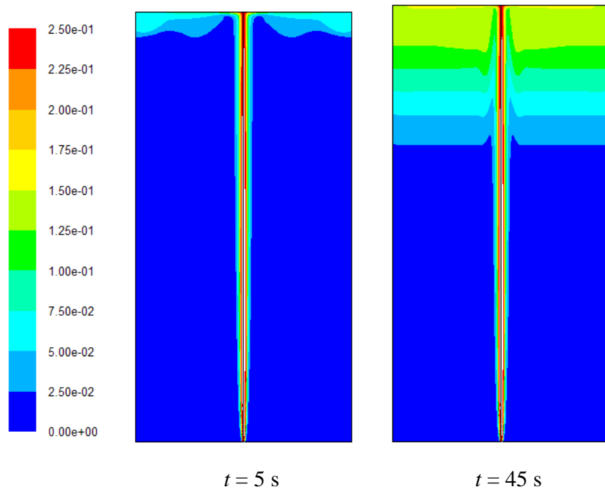
Figure 2. Hydrogen mole fraction contours at different times for a 2-mm-diameter leak at the cylinder bottom with Re = 1000
