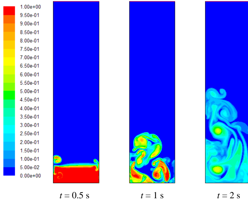
Figure 1. Hydrogen mole fraction contours for open top cylinder at different times
