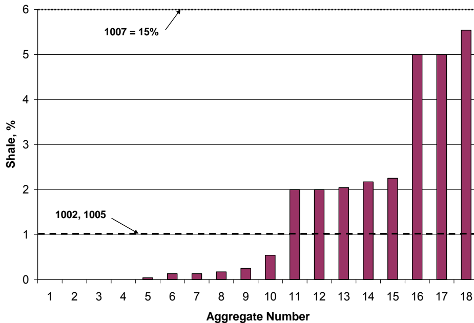
Figure 4: Distribution of Shale in Samples
