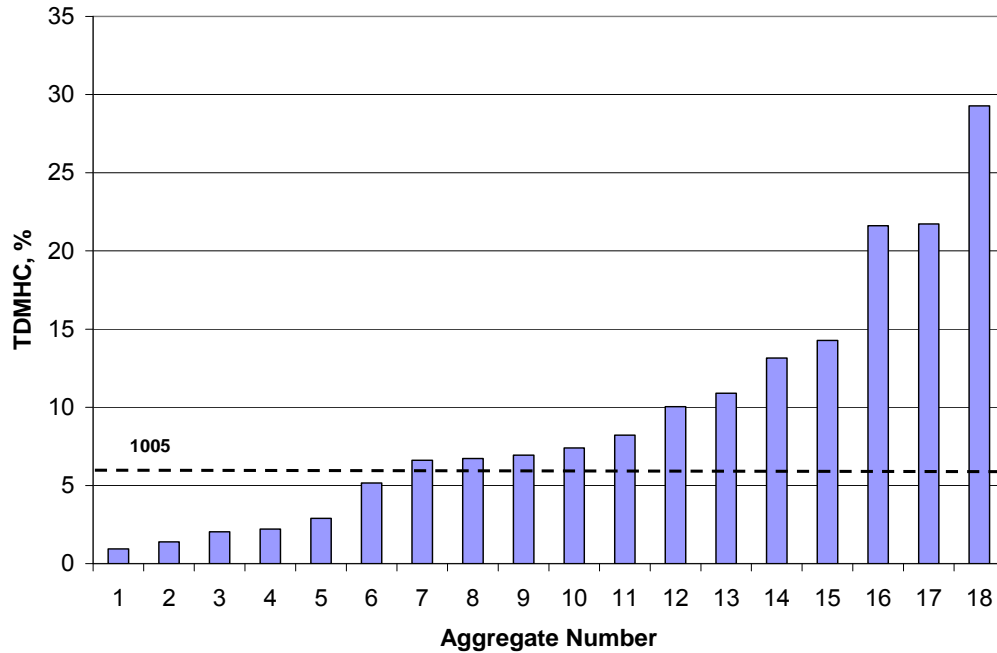
Figure 7: Distribution of Total Deleterious Material Hard Chert in Samples
