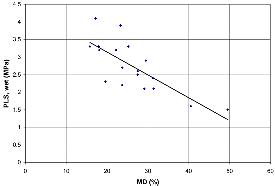
Figure 24: Micro-Deval vs. Point Load Strength wet
