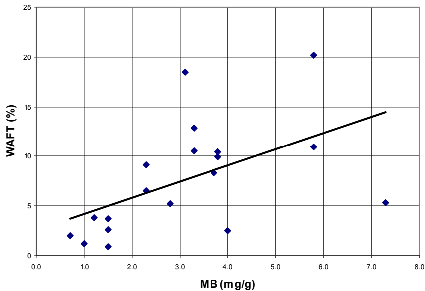
Figure 24: Water Alcohol Freeze-Thaw Soundness vs. Methylene Blue
