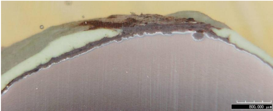
(c) Corrosion detail at d-d section
