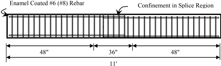
(b) With confinement in the splice region
