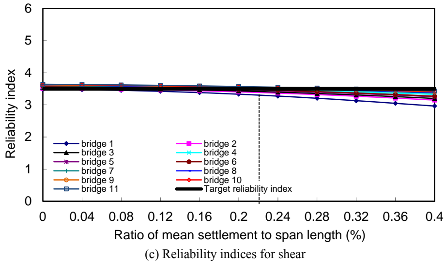
Figure 5.22 Reliability indices of 3-span bridges (No.12 to No.22 in Table 2.3): Case 7
