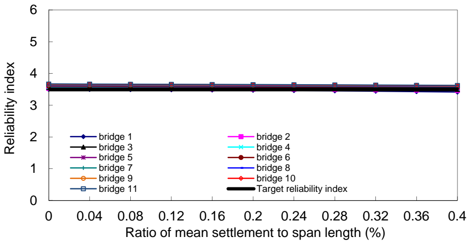
Figure 5.21 Reliability indices of 2-span bridges (No.1 to No.11 in Table 2.3): Case 7
