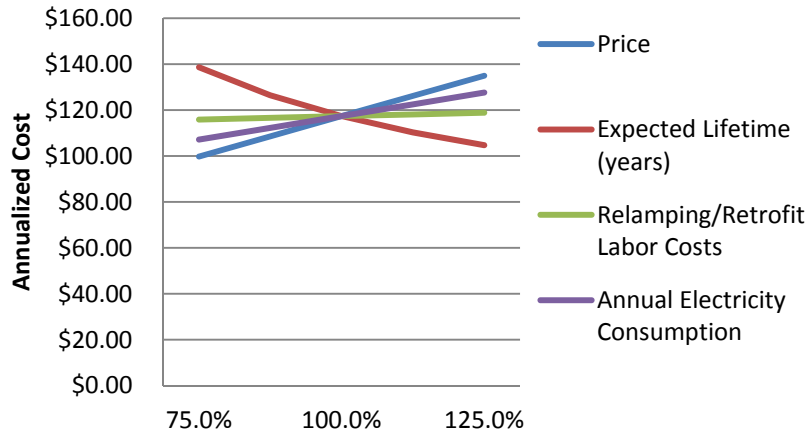
Figure 19 – Sensitivity Analysis of Dialight Luminaire
