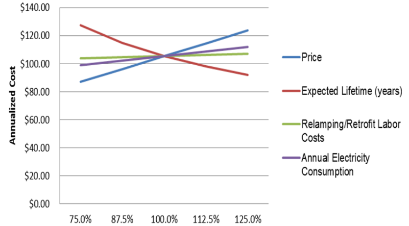
Figure 20 - Sensitivity Analysis of 250 W HPS
